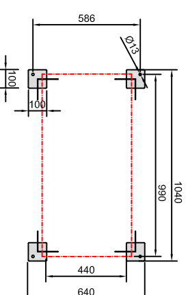
HUELLAS / SUPPORTS
